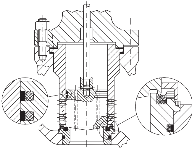
Fig. 10 Quick-change seat – Soft seat insert – Piston ring – Bal. trim
