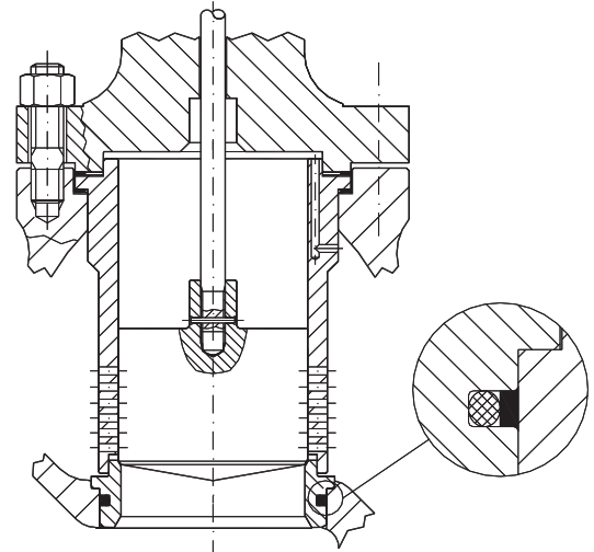
Fig. 13 Quick-change seat – Unbalanced trim
