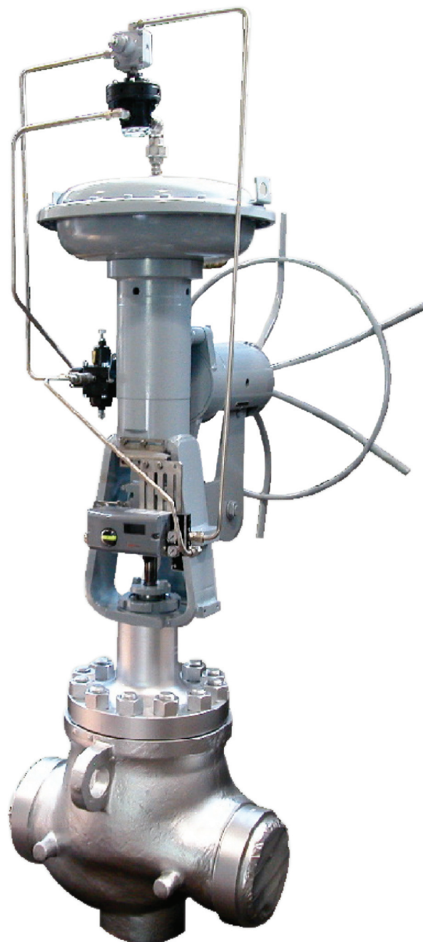
Fig. 1 Valve Model CH/L Globe Valve 8" ANSI 600 with pneumatic actuator
