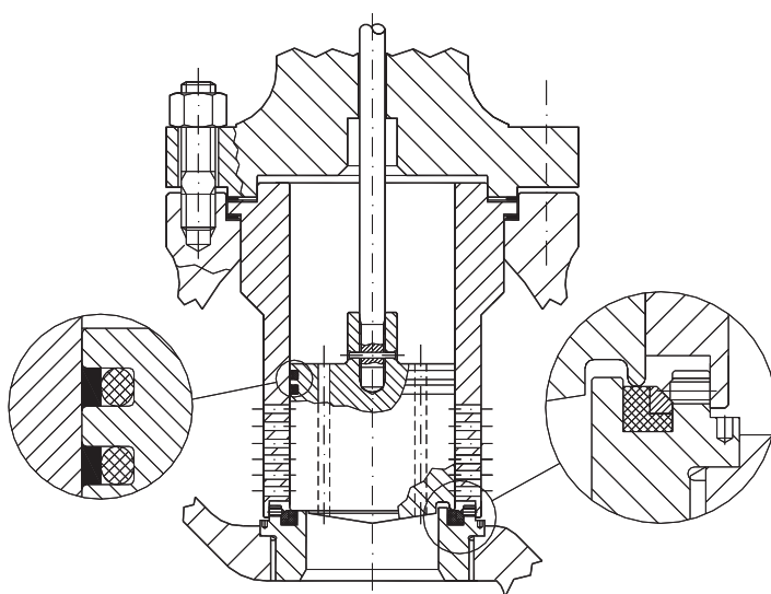
Fig. 6 Threaded seat – Soft seat insert – Balanced trim
