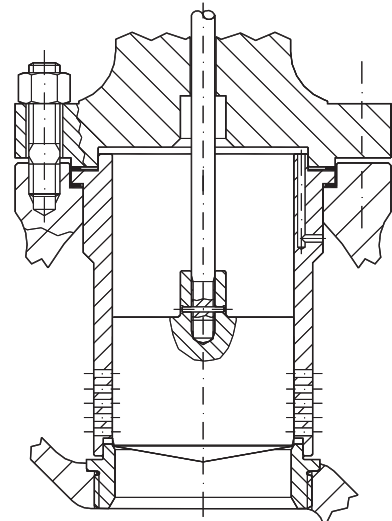
Fig. 9 Threaded seat – Unbalanced trim
