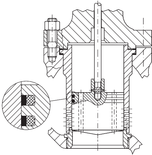
Fig. 8 Threaded seat – Piston ring – Balanced trim
