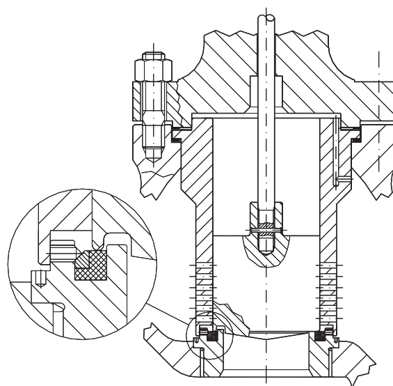
Fig. 7 Threaded seat – Soft seat insert – Unbalanced trim
