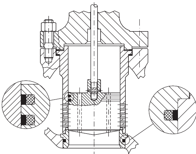
Fig. 12 Quick-change seat - Balanced trim
