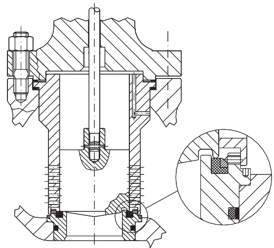
Fig. 11 Quick-change seat – Soft seat insert – Unbalanced trim
