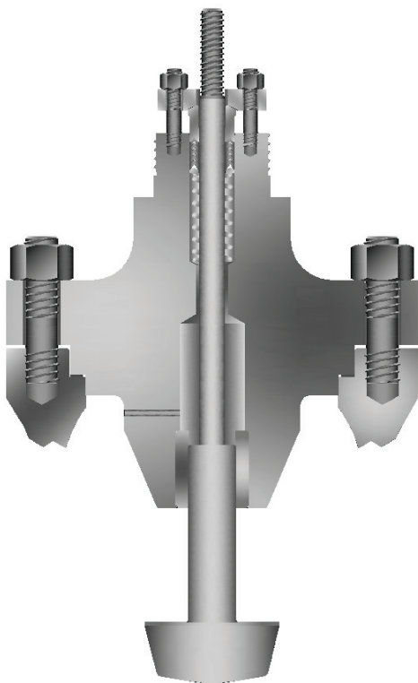
Fig. 4 Standard bonnet for unbalanced trim
