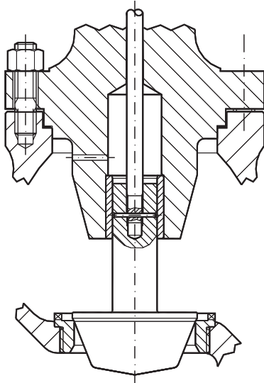
Fig. 7 Threaded seat, Unbalanced trim
