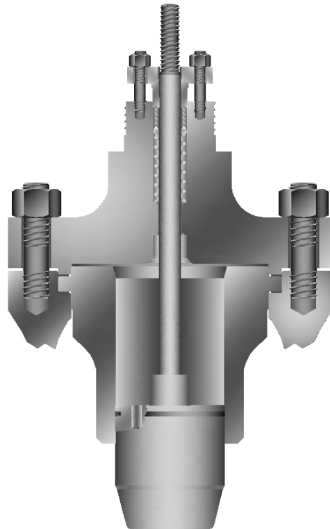
Fig. 5 Standard bonnet for balanced trim
