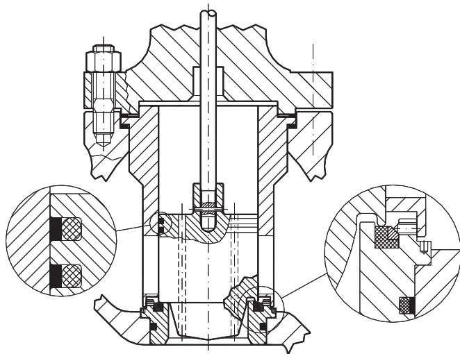
Fig. 13 Quick change seat, soft seat insert, Balanced trim
