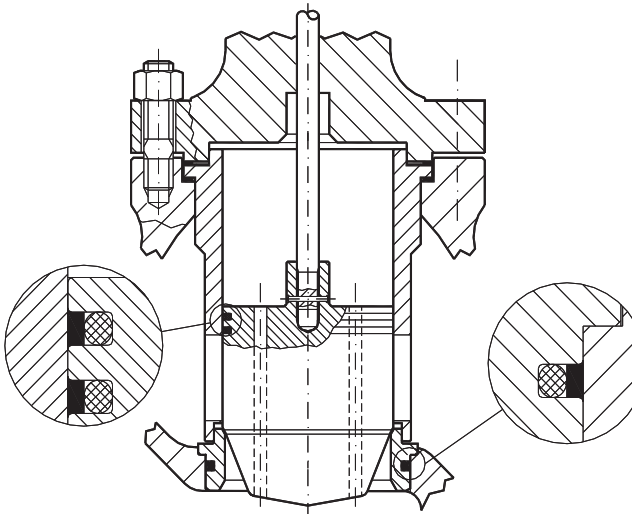
Fig. 11 Quick change seat, Balanced trim
