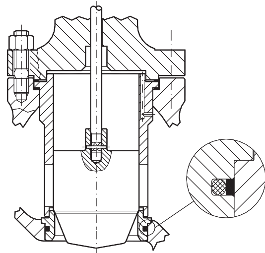
Fig. 10 Quick change seat, Unbalanced trim
