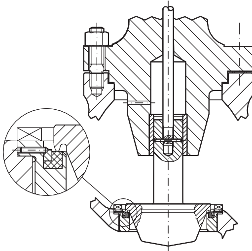
Fig. 9 Threaded seat, soft seat insert, Unbalanced trim
