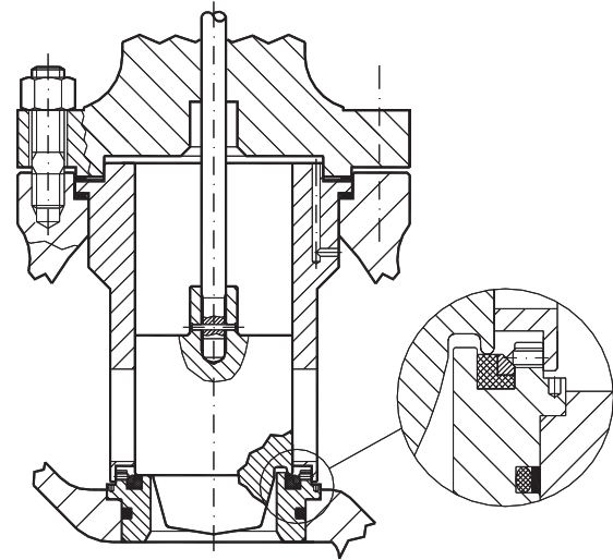
Fig. 12 Quick change seat, soft seat insert, Unbalanced trim
