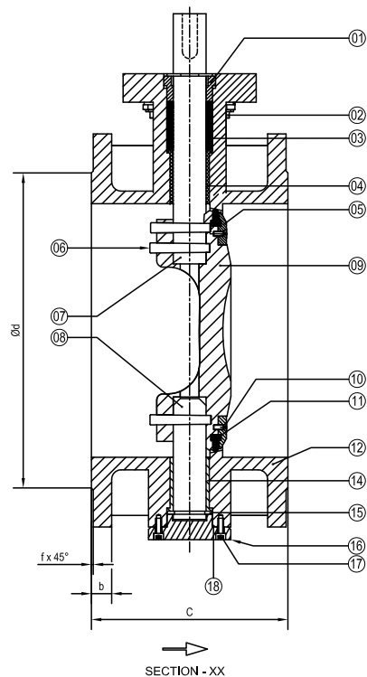
SECTION - XX
