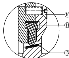
SECTION - XX
